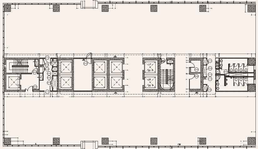
Floor Plan
